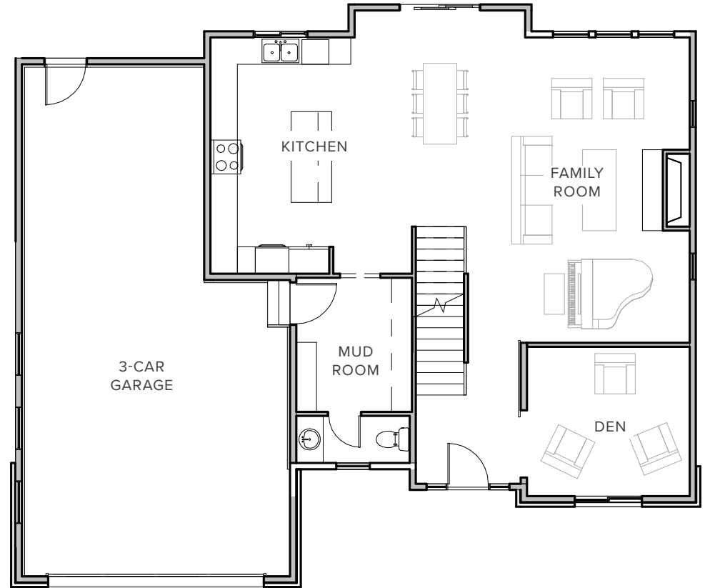
MAIN LEVEL
